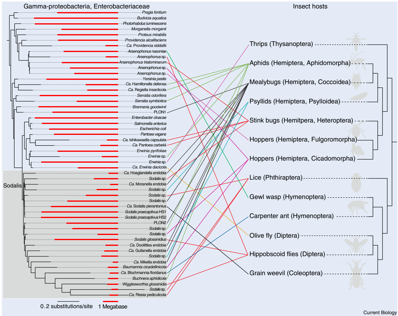
Figure 2. The tangled evolutionary relationships of selected HBEs, their diverse insect hosts, and the range of genome sizes. Bacterial genome sizes are shown as red bars. The colored lines connect insect groups to known bacterial symbionts. The Enterobacteriaceae phylogeny is based on maximum likelihood analysis of 130 concatenated protein-coding genes from 93 taxa (database construction, tree search, model fitting, and tree refinement methods can be found in the Supplemental Information). The insect phylogeny was adapted from [1]. Ca. = Candidatus , PLON = Pseudococcus longipinus symbiont, sp. = species.
